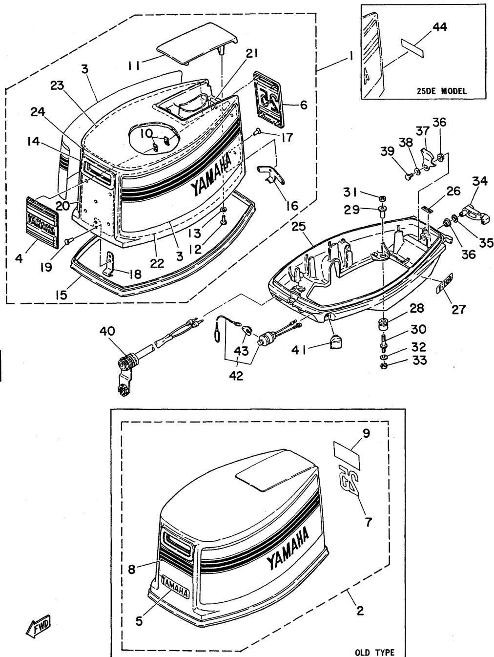
Fig. 2 COWLING '80/'81
