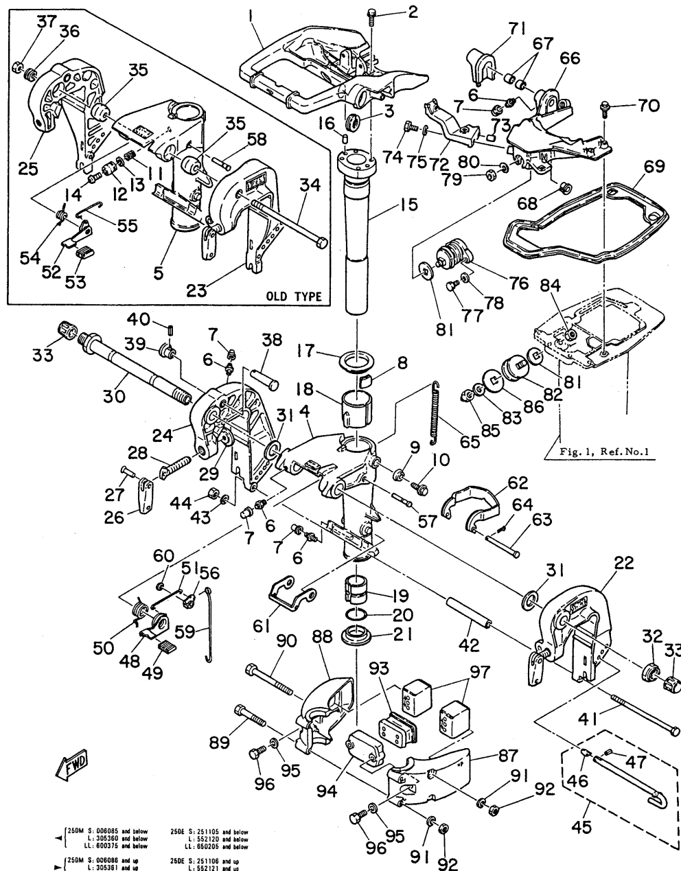
Fig. 12 BRACKET '80/'81
