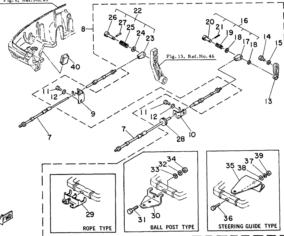
Fig. 2, Ref. No. 25
