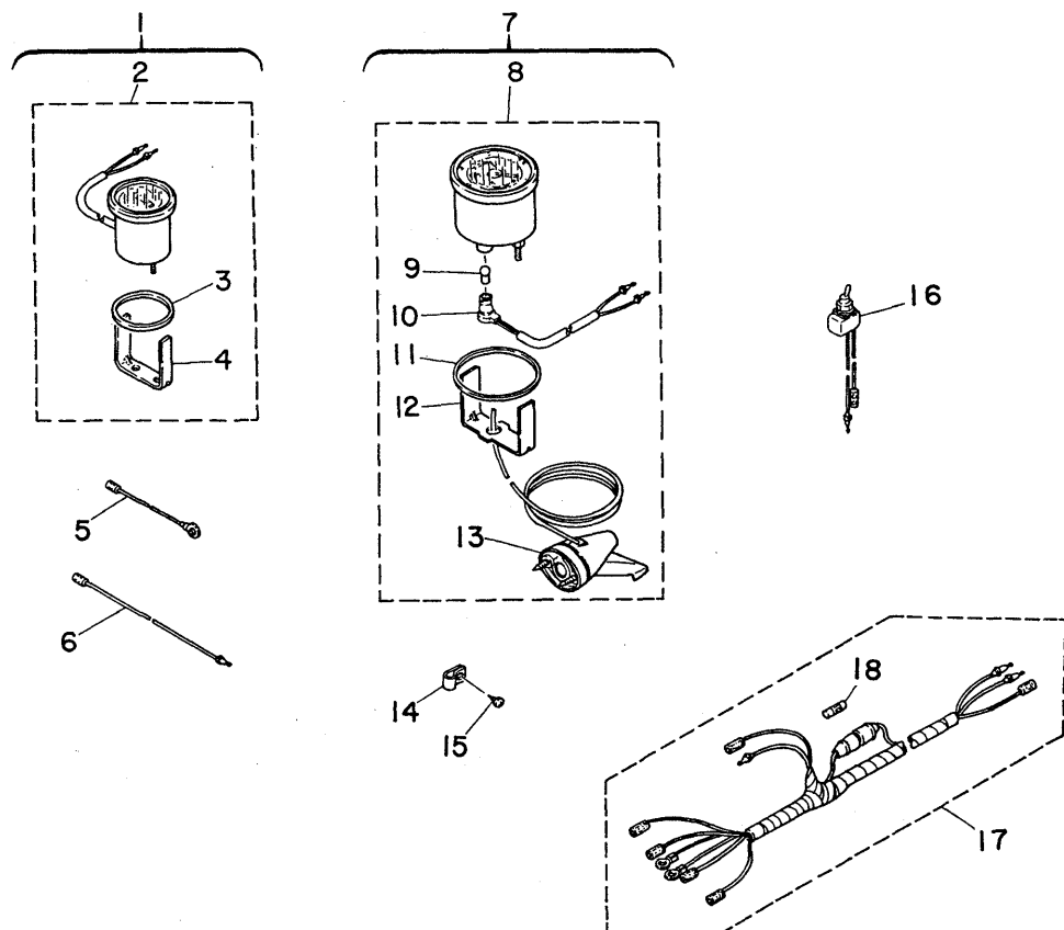
Fig.24 ACCESSORY PARTS 2 -'80/'81
