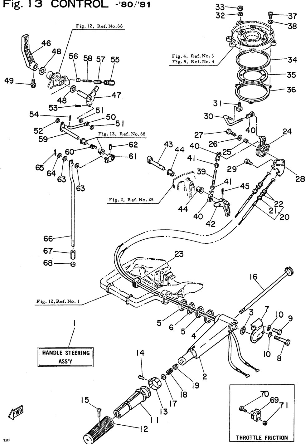
Fig. 13 CONTROL -'80/'81
