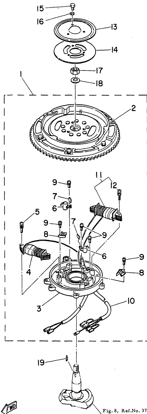
Fig. 4 FLYWHEEL MAGNETO (80W) -'80/'81
