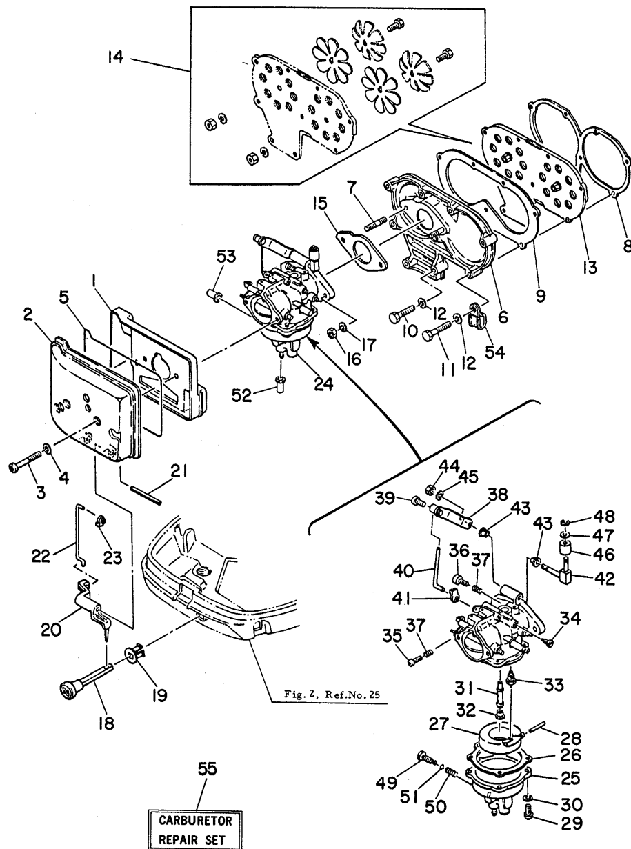
Fig. 9 INTAKE -'80/'81
