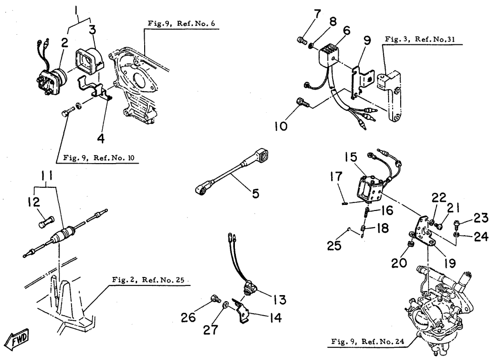
Fig. 17 ELECTRIC PARTS (25DE MODEL) -'80/'81
