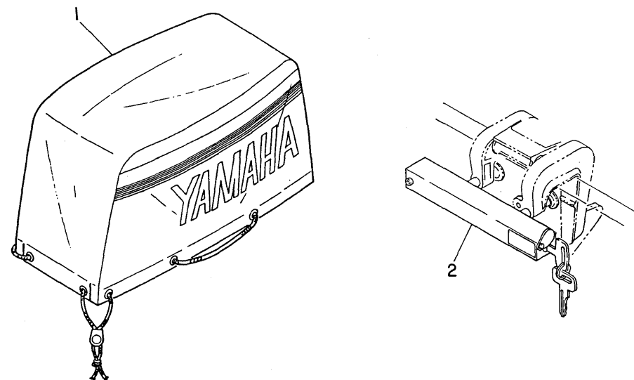
Fig.25 ACCESSORY PARTS 3 -'80/'81
