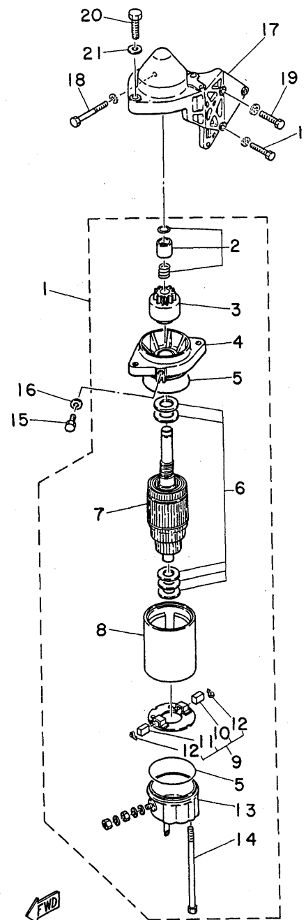
Fig. 16 ELECTRIC MOTOR (25DE MODEL) -'80/'81
