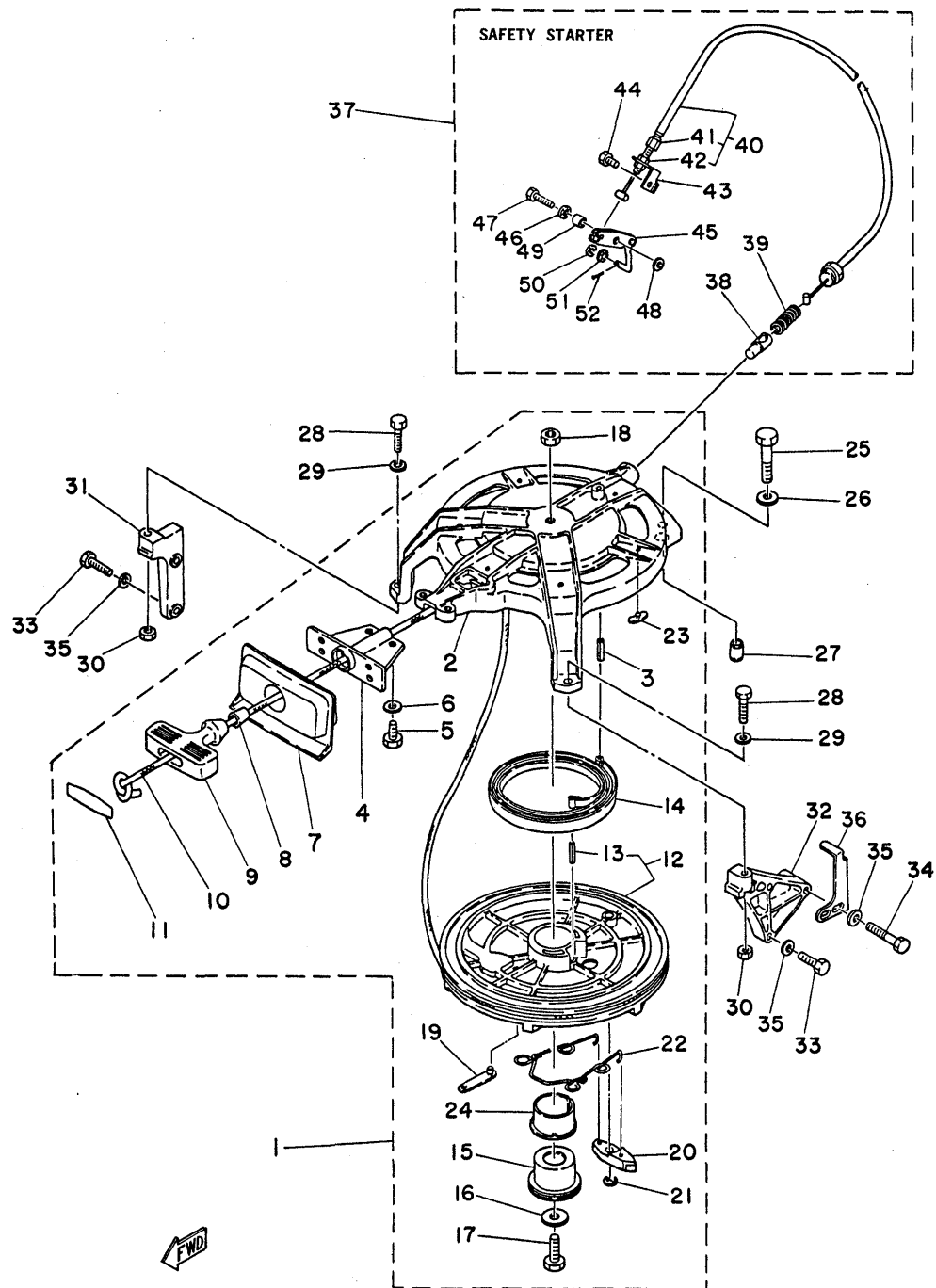
Fig. 3 STARTER '80/'81
