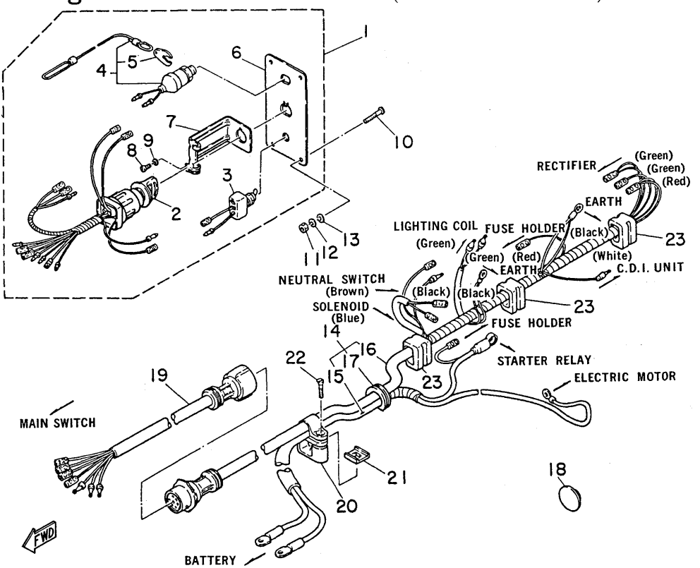
Fig. 18 SWITCH PANEL (25DE MODEL) -'80/'81
