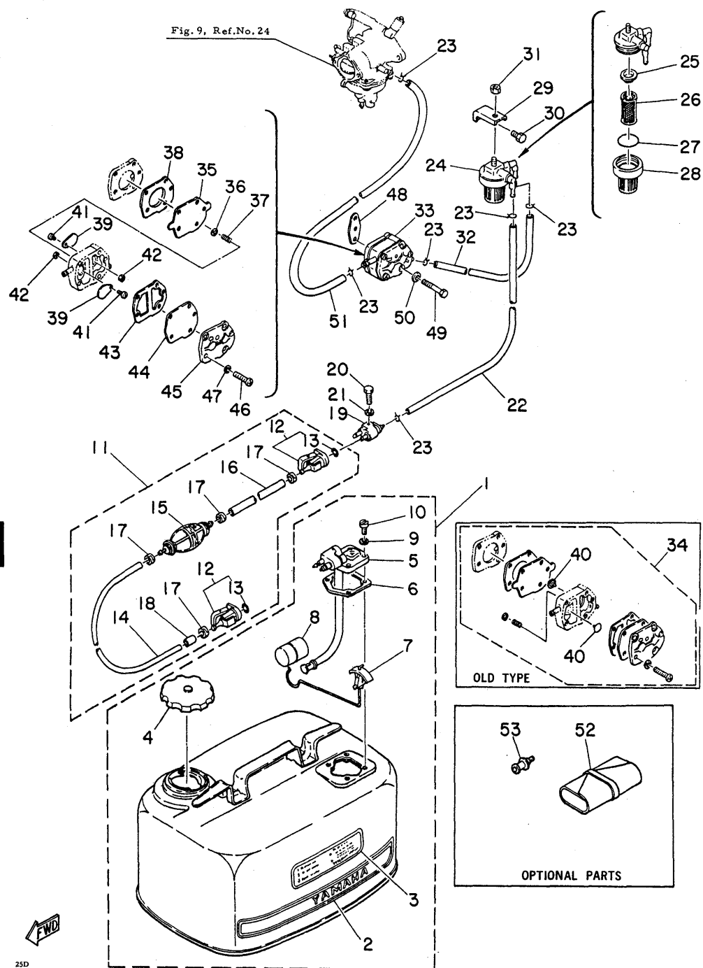
Fig. 14 FUEL SECTION -'80/'81
